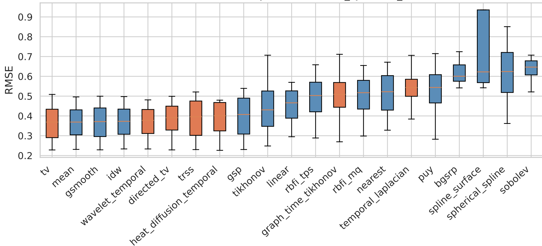
RMSE Distribution by Method — it03_synthetic_beta
