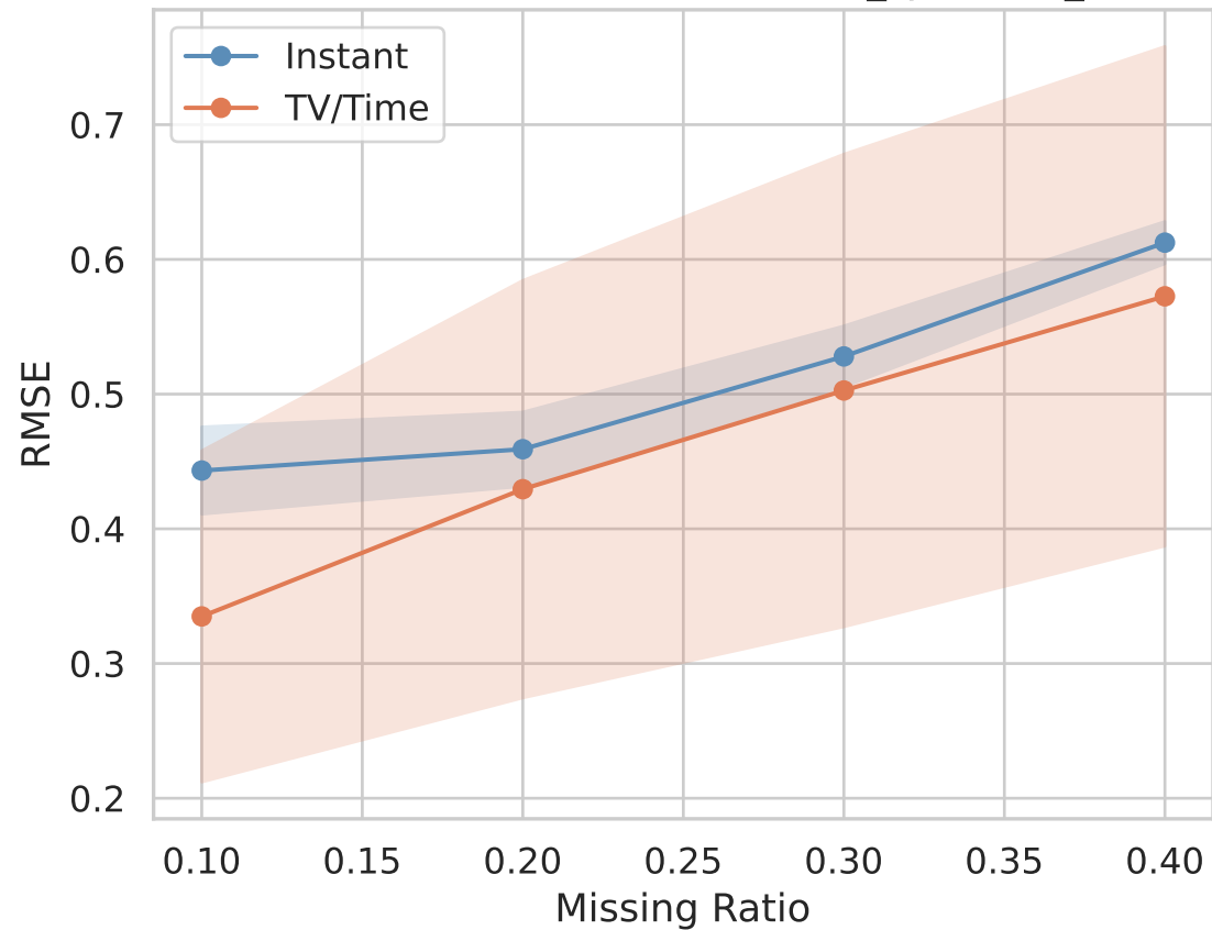
RMSE — TV/Time vs Instant — it03_synthetic_beta
