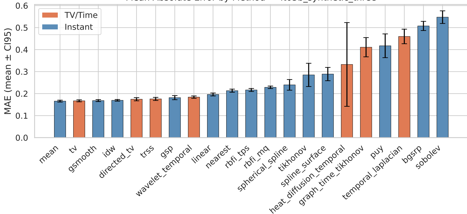
Mean Absolute Error by Method — it05b_synthetic_three
