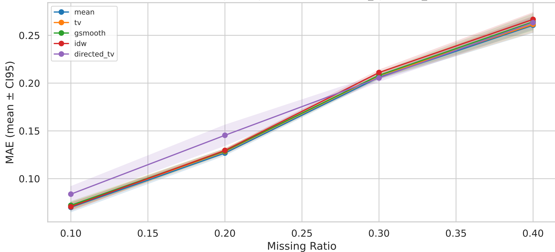
MAE Sensitivity — Top-5 Methods — it05b_synthetic_three
