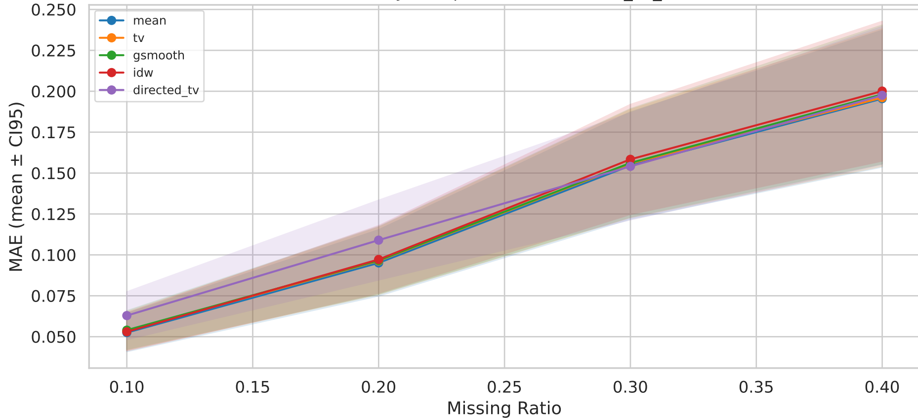
MAE Sensitivity — Top-5 Methods — it05_all_datasets
