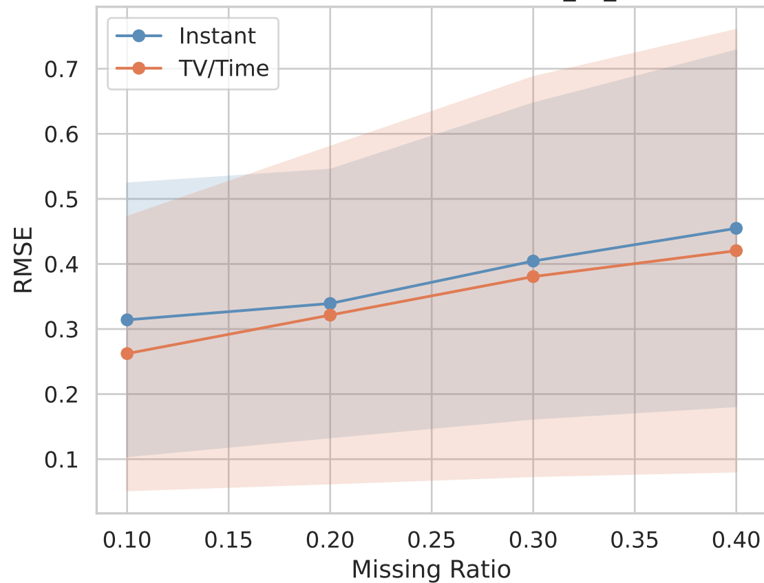
RMSE — TV/Time vs Instant — it05_all_datasets
