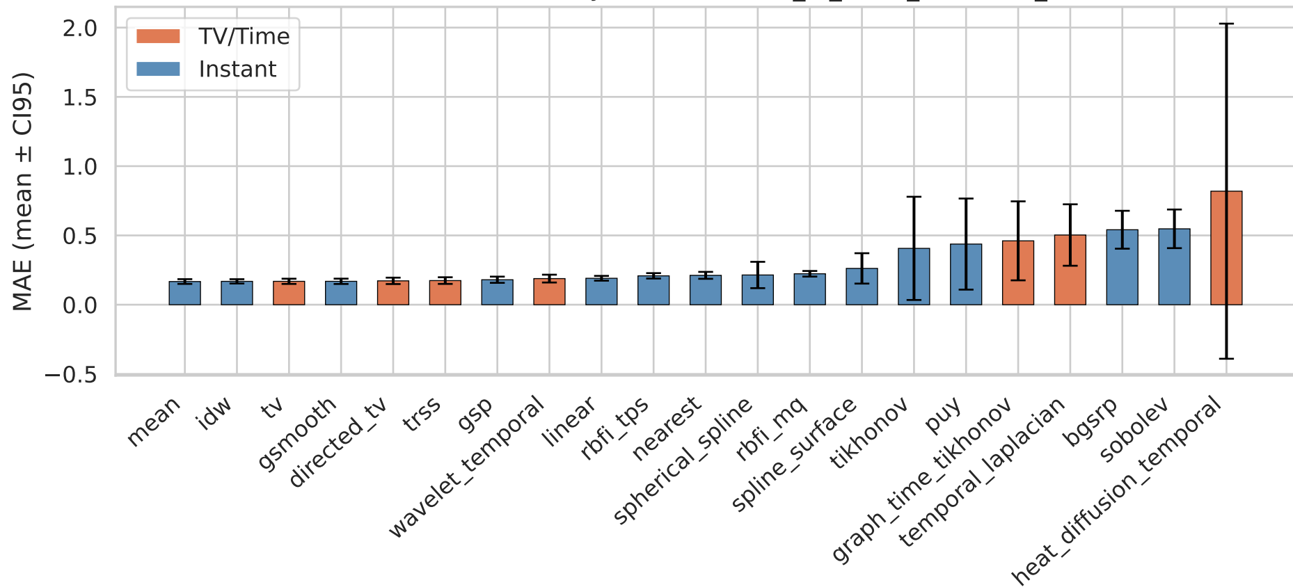
Mean Absolute Error by Method — it06_tv_focus_kalofolias_nnk
