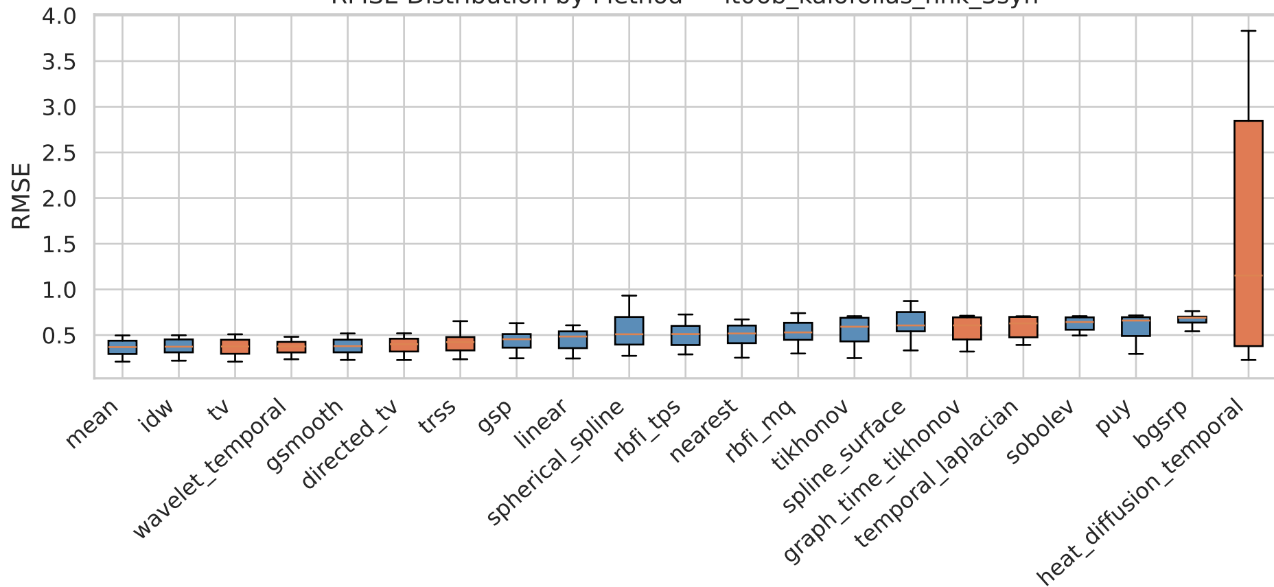
RMSE Distribution by Method — it06b_kalofolias_nnk_3syn
