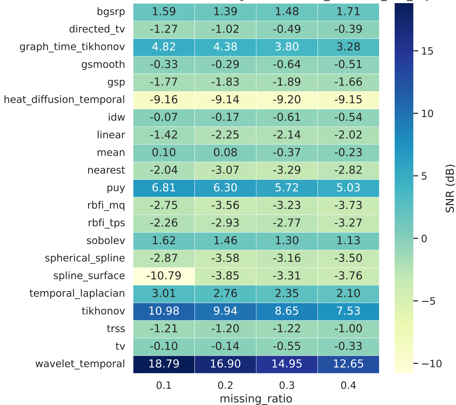
Mean SNR — Method × Missing Ratio — it06b_kalofolias_nnk_3syn
