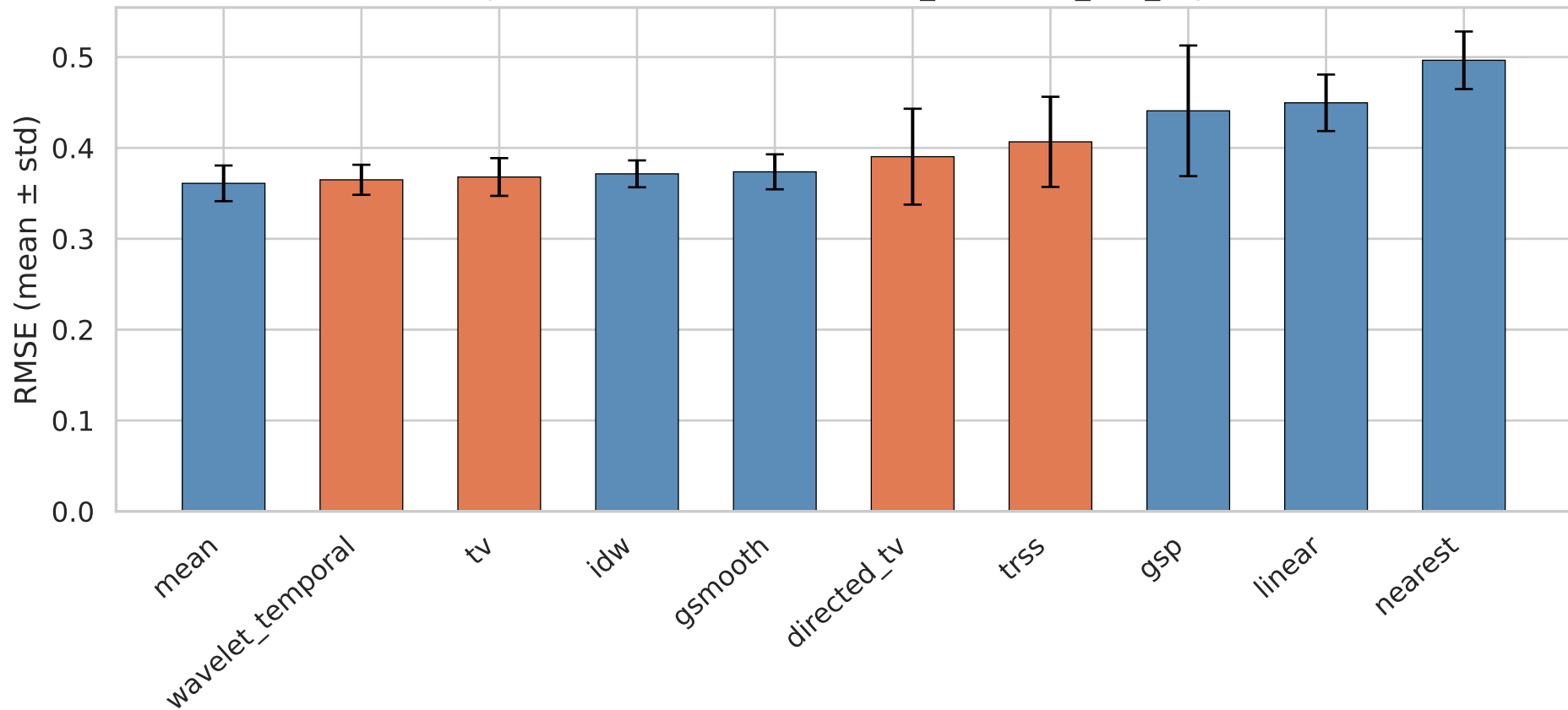
Top-10 Methods: RMSE — it06b_kalofolias_nnk_3syn
