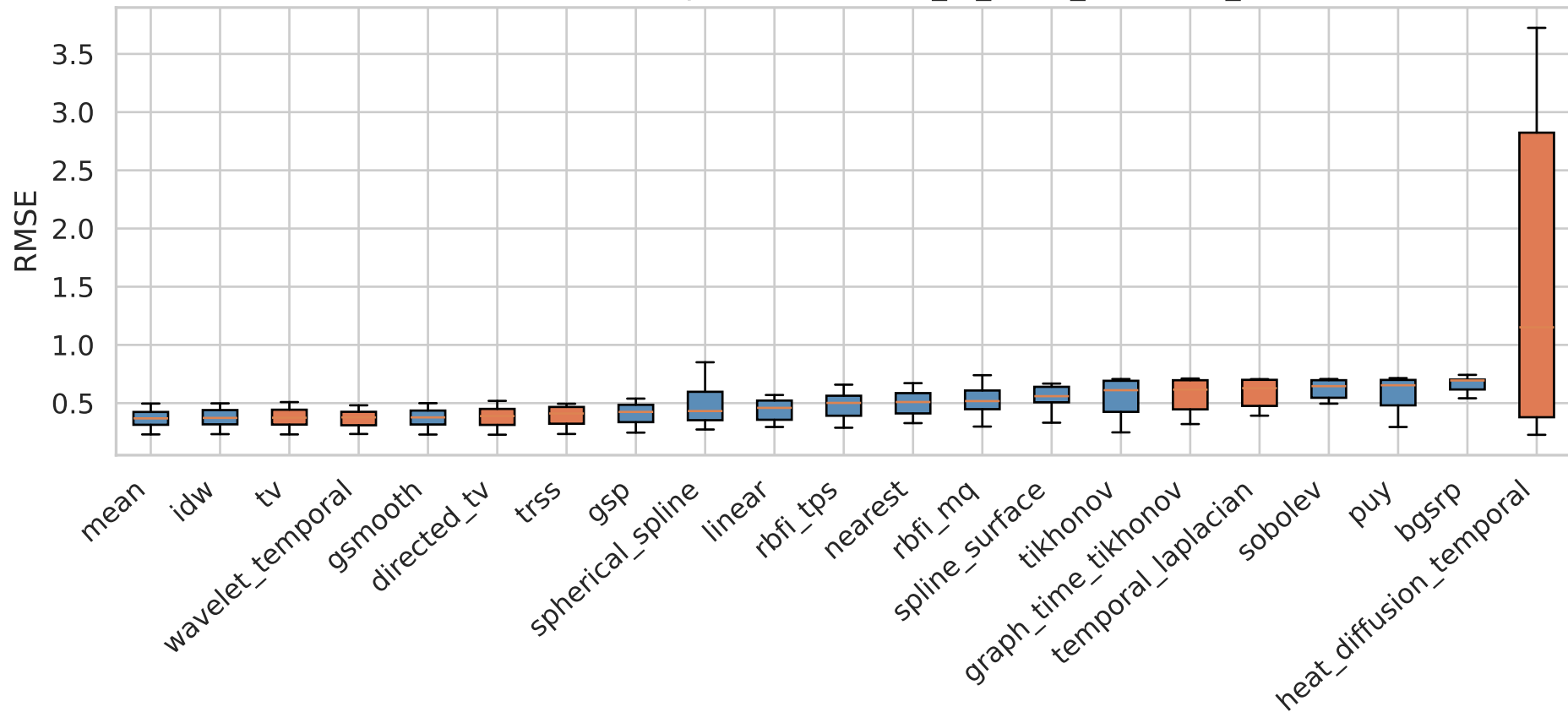
RMSE Distribution by Method — it06_tv_focus_kalofolias_nnk
