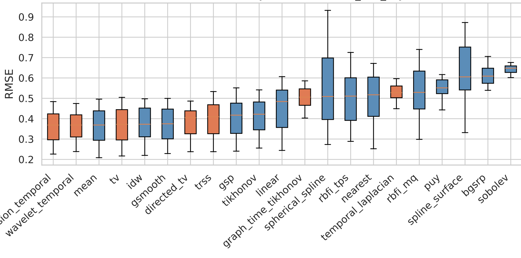
RMSE Distribution by Method — it07b_knn_3syn
