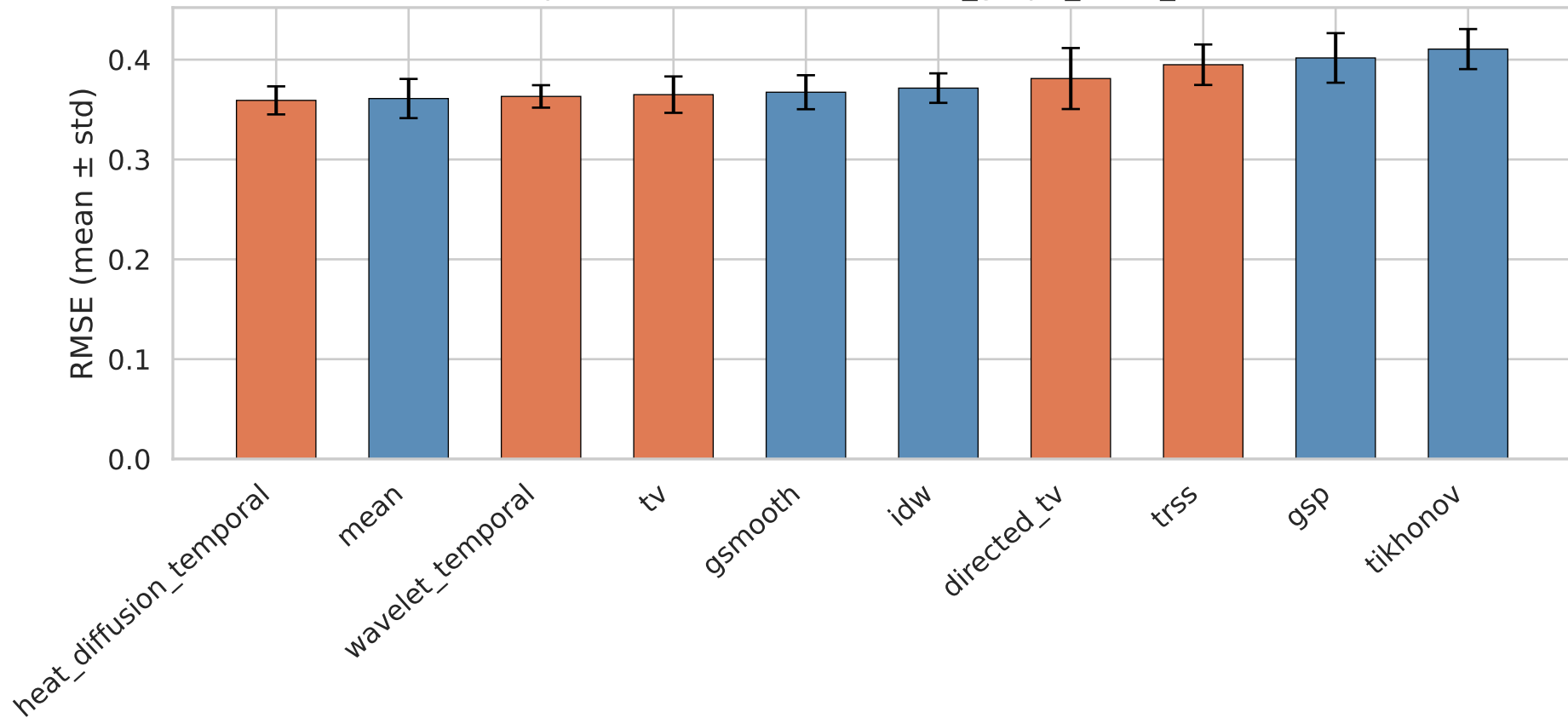
Top-10 Methods: RMSE — it07_graph_focus_knn
