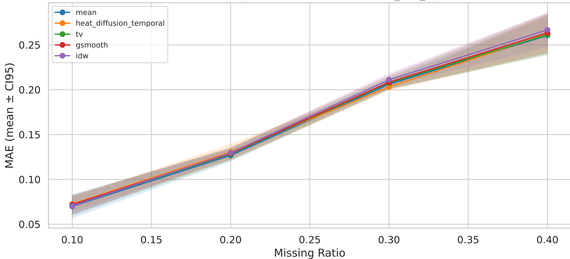
MAE Sensitivity — Top-5 Methods — it07b_knn_3syn
