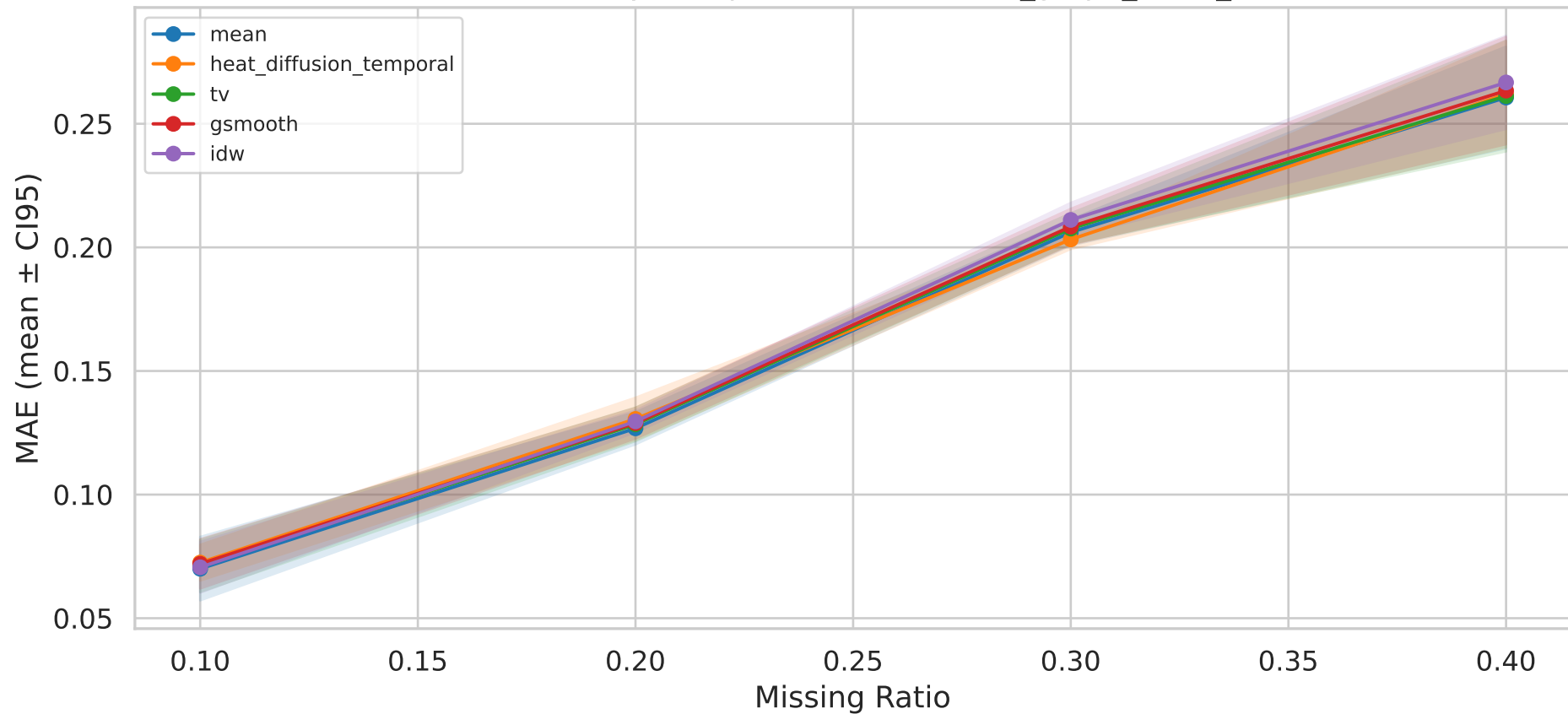
MAE Sensitivity — Top-5 Methods — it07_graph_focus_knn
