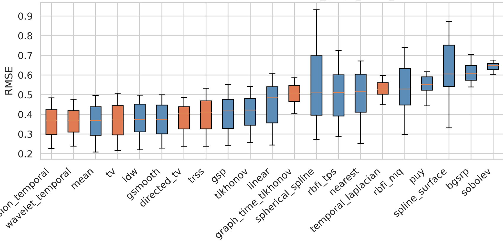
RMSE Distribution by Method — it07_graph_focus_knn
