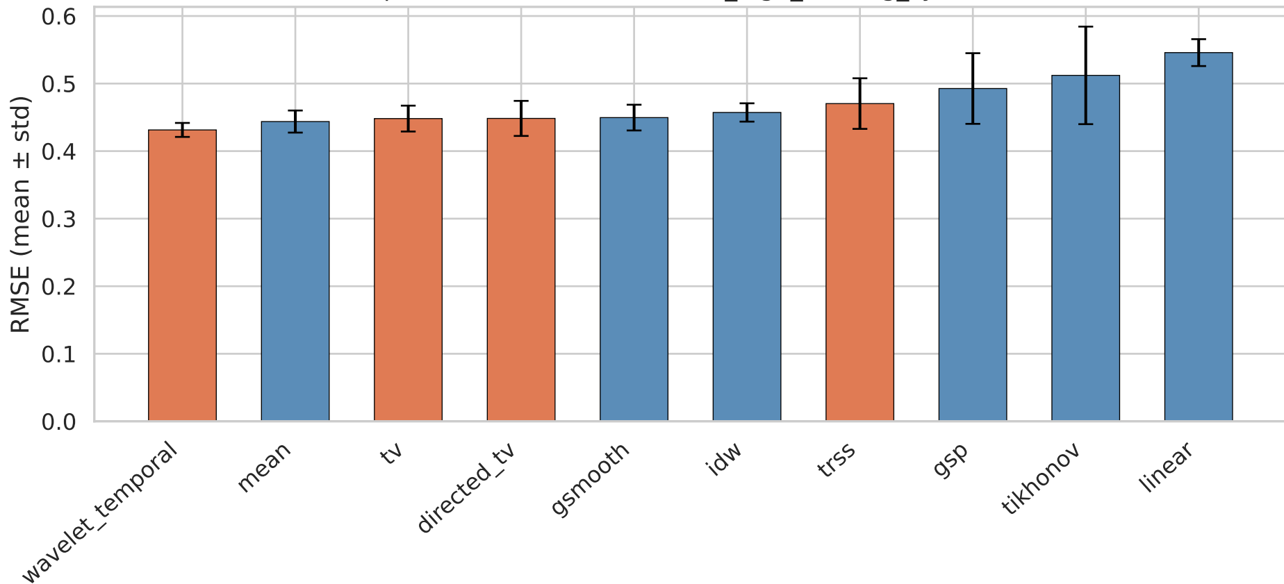
Top-10 Methods: RMSE — it08_high_missing_synthetic
