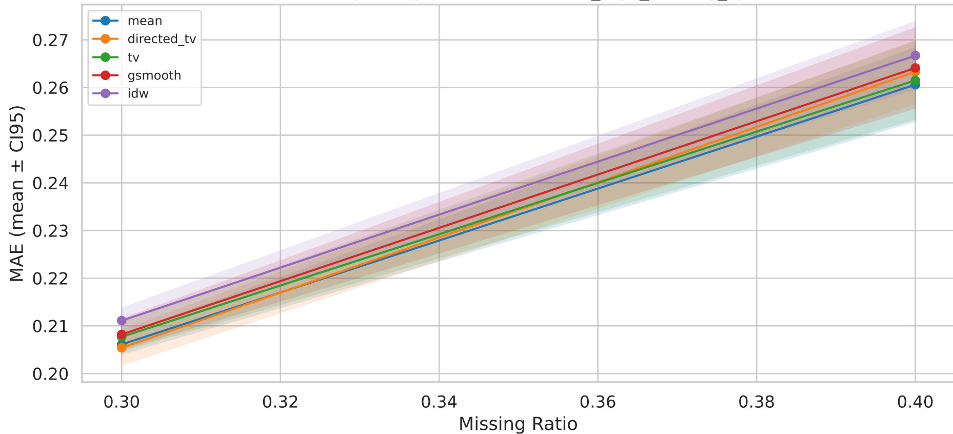
MAE Sensitivity — Top-5 Methods — it08_high_missing_synthetic
