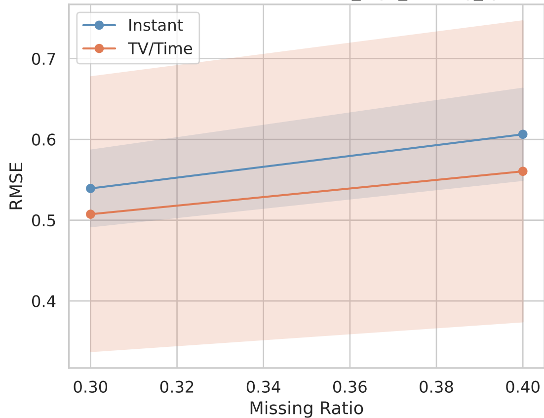
RMSE — TV/Time vs Instant — it08_high_missing_synthetic
