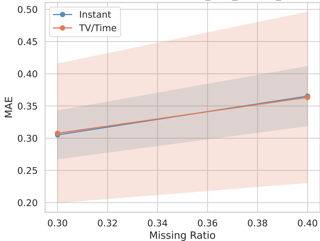
MAE — TV/Time vs Instant — it08_high_missing_synthetic
