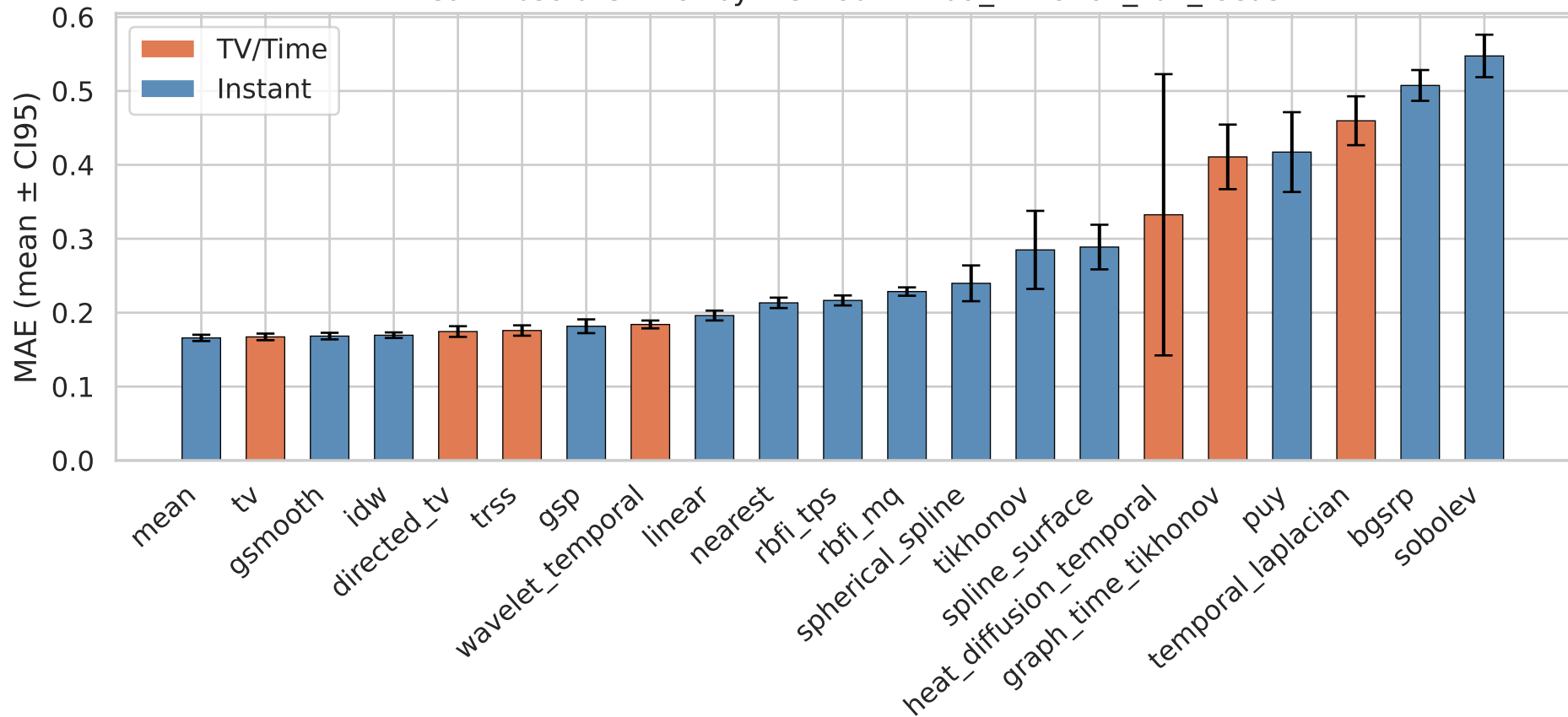
Mean Absolute Error by Method — it09_tikhonov_rbfi_focus
