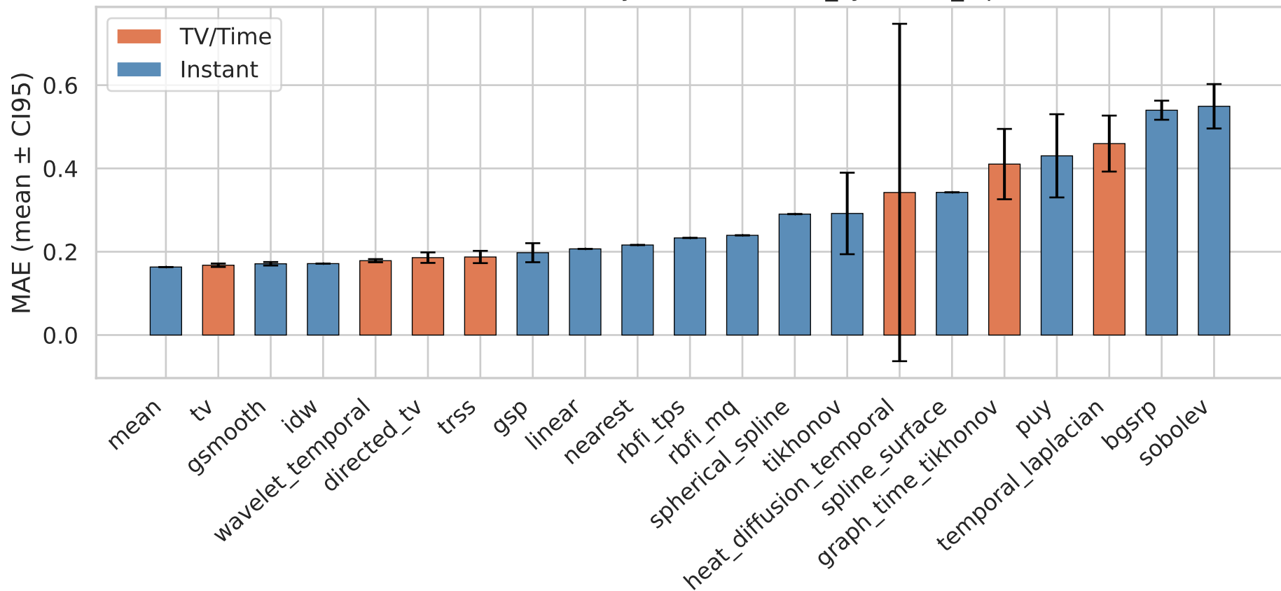
Mean Absolute Error by Method — it10_synthetic_alpha
