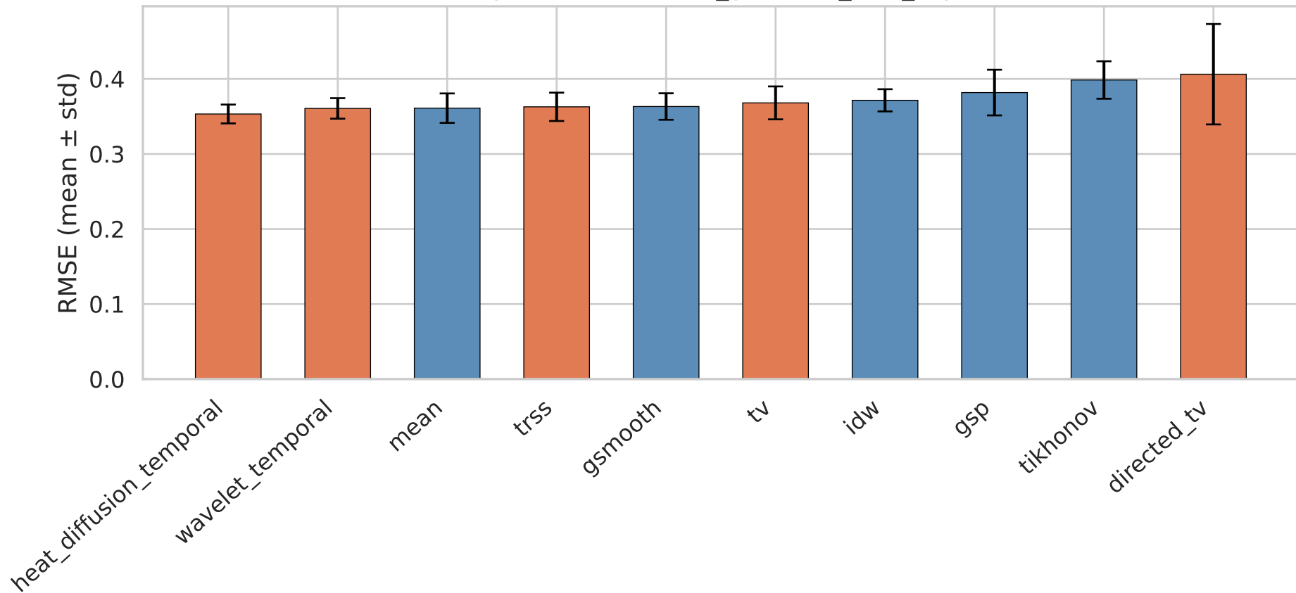
Top-10 RMSE — it13_gaussian_aew_3syn
