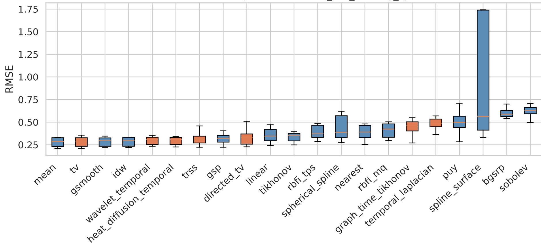
RMSE Distribution by Method — it14_low_missing_synthetic
