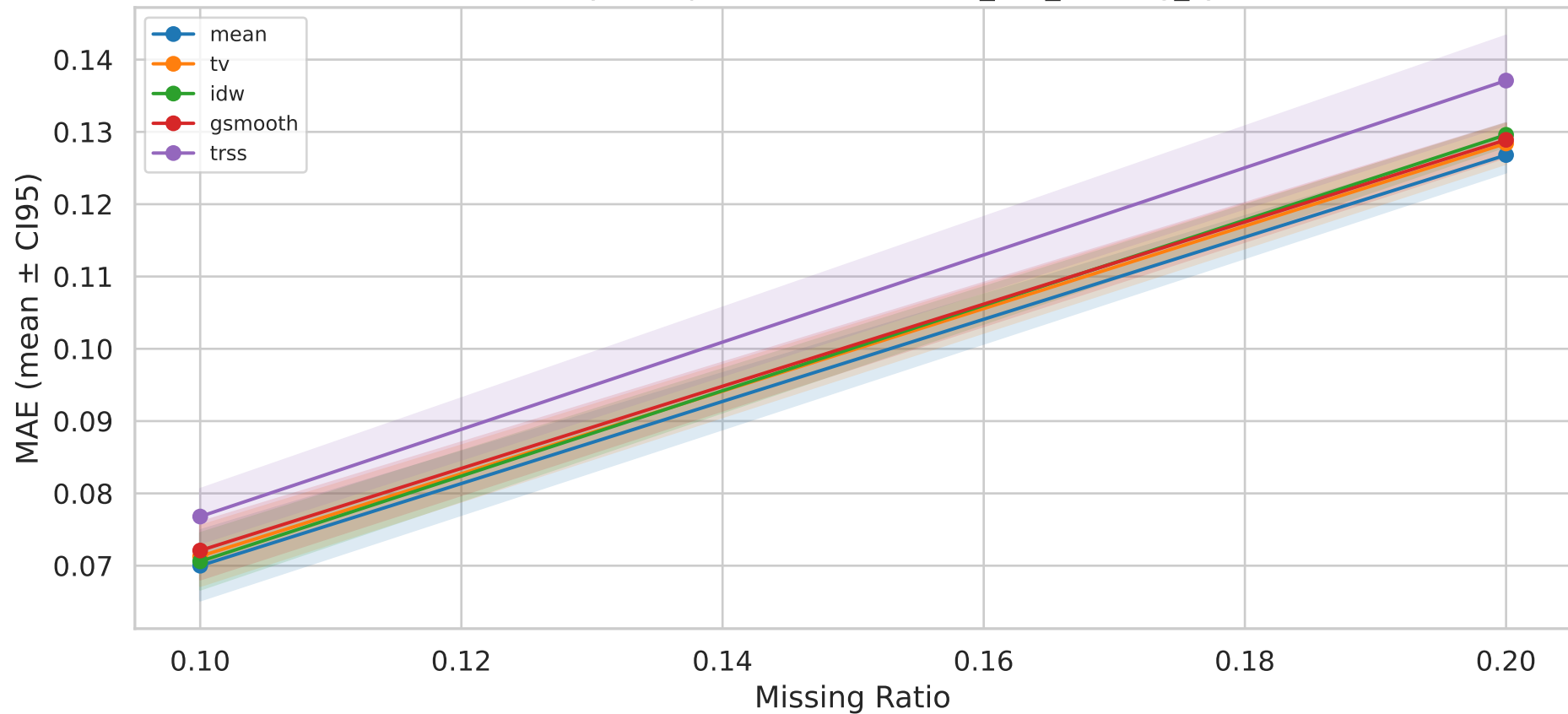
MAE Sensitivity — Top-5 Methods — it14_low_missing_synthetic
