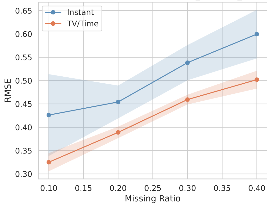
RMSE — TV/Time vs Instant — it15b_gaussian_3syn
