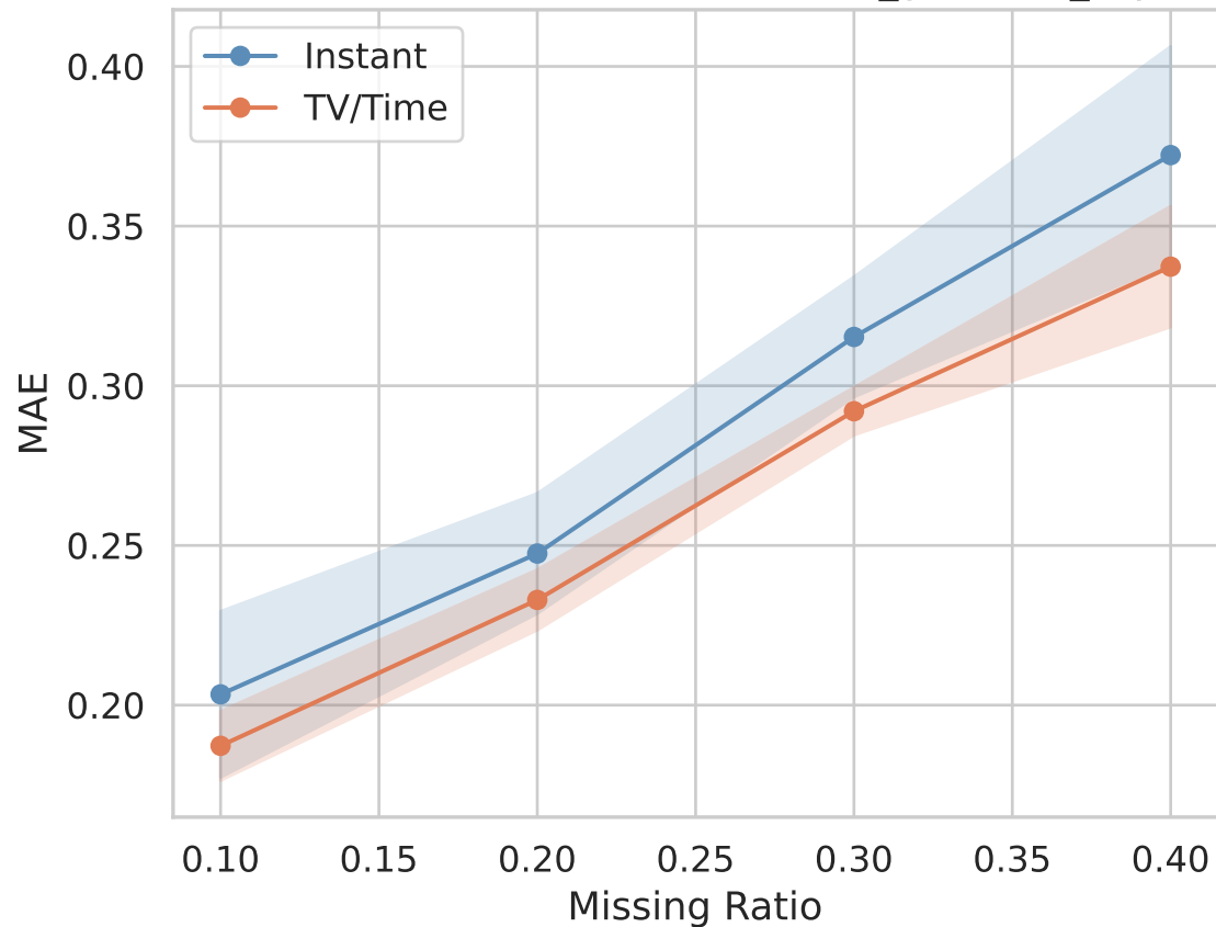
MAE — TV/Time vs Instant — it15b_gaussian_3syn
