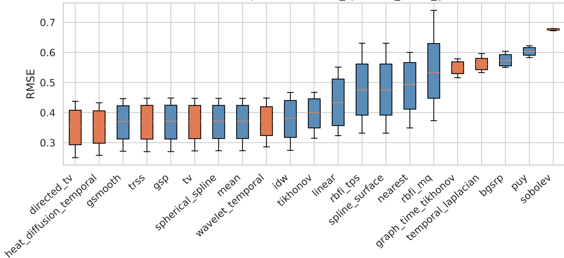
RMSE Distribution by Method — it15_synthetic_broad_gaussian
