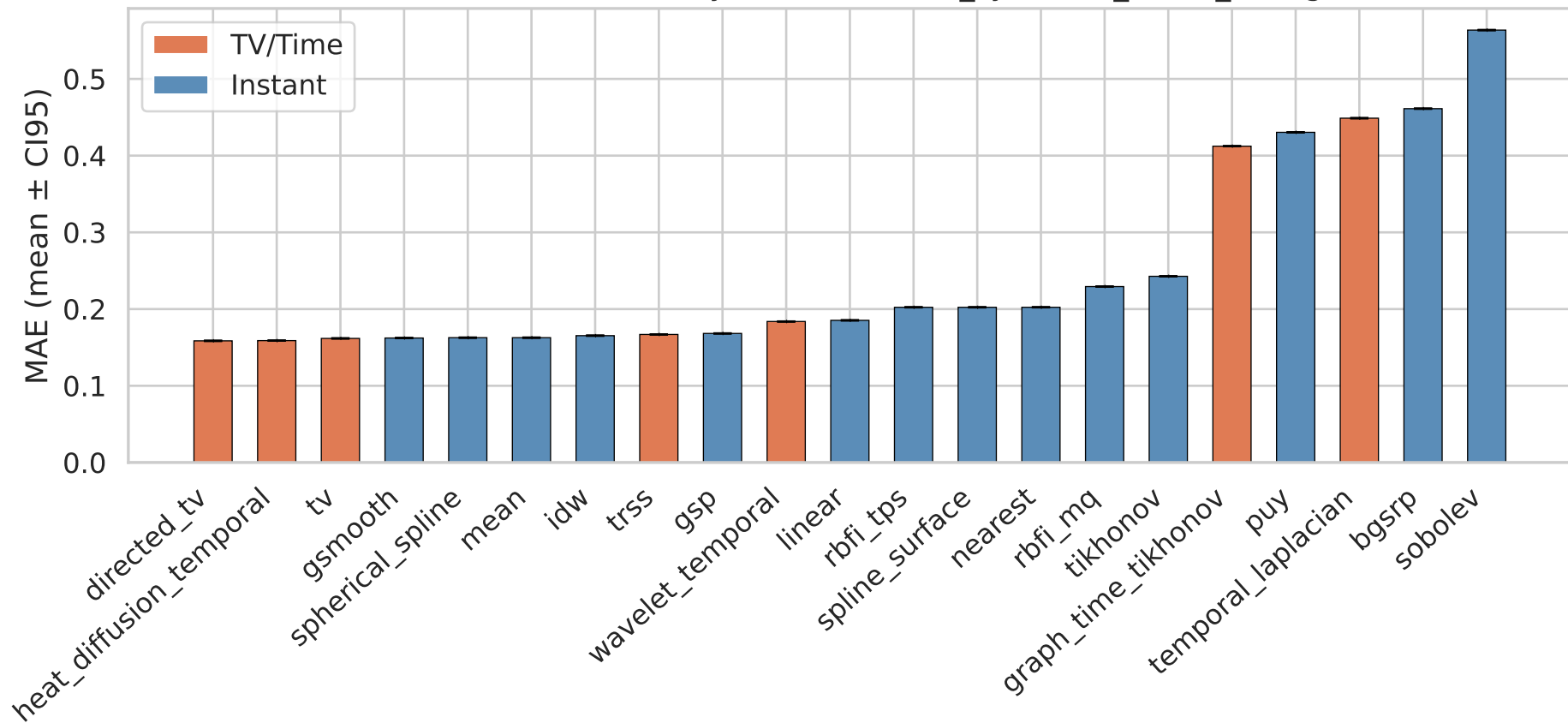
Mean Absolute Error by Method — it16_synthetic_broad_vknnng
