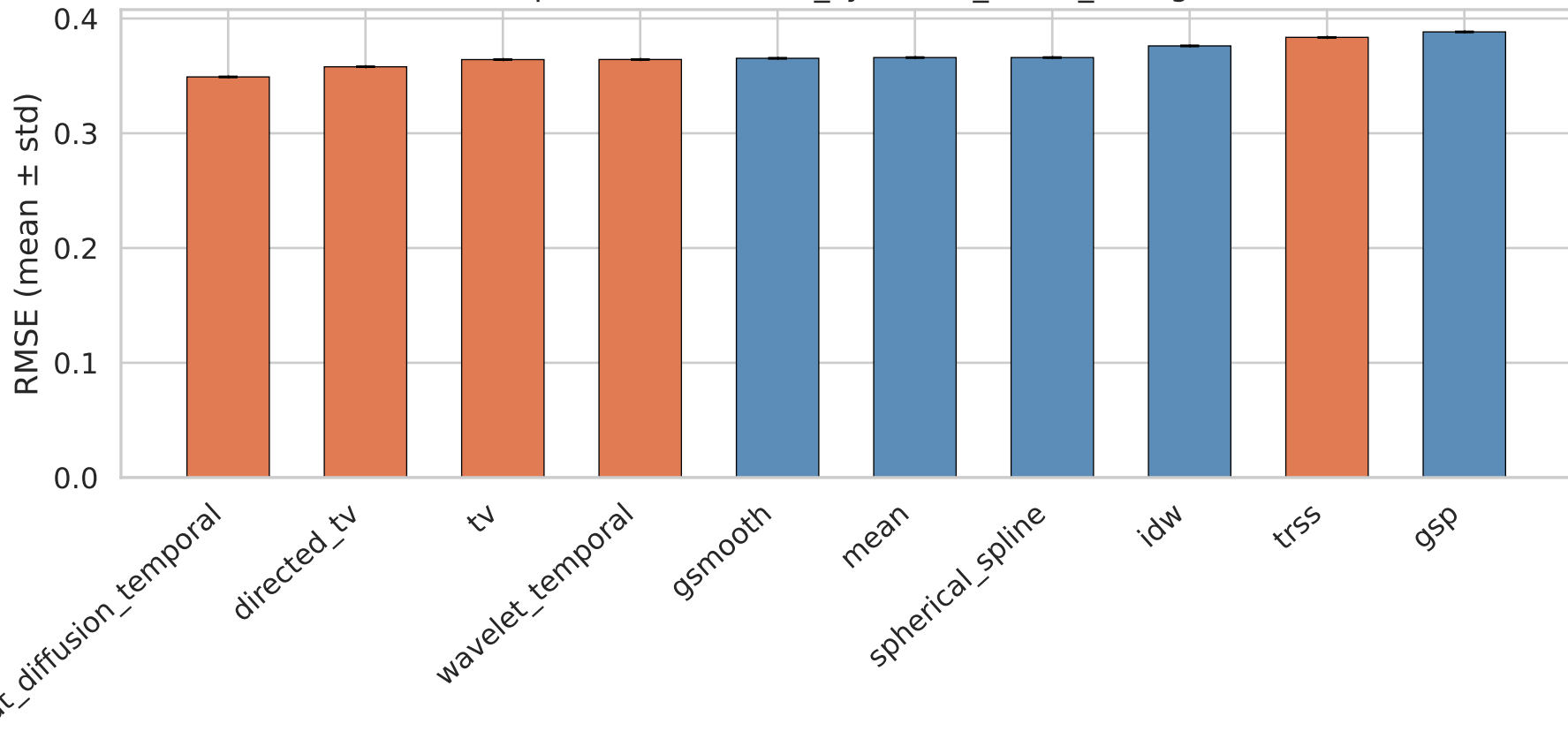
Top-10 RMSE — it16_synthetic_broad_vknnng
