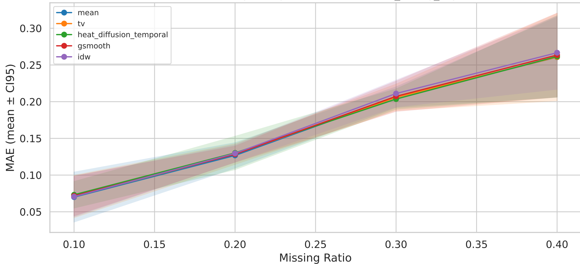
MAE Sensitivity — Top-5 Methods — it16b_vknnng_3syn
