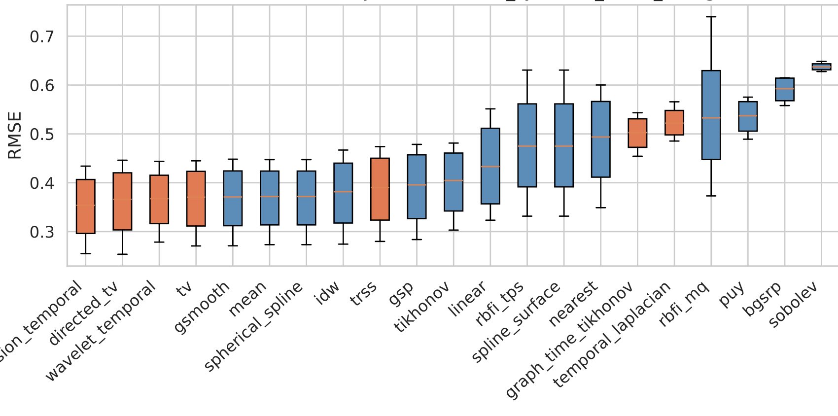
RMSE Distribution by Method — it16_synthetic_broad_vknnng
