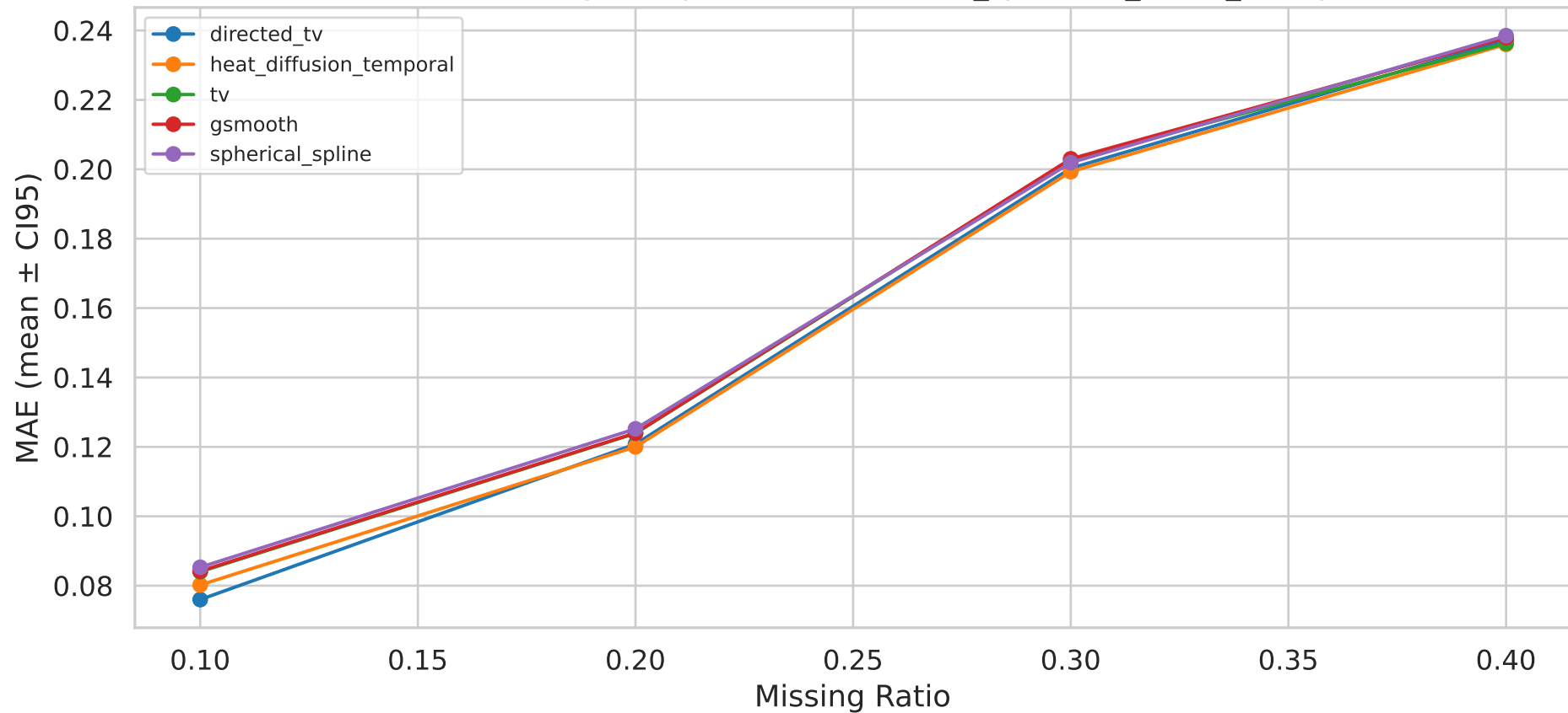
MAE Sensitivity — Top-5 Methods — it16_synthetic_broad_vknnng
