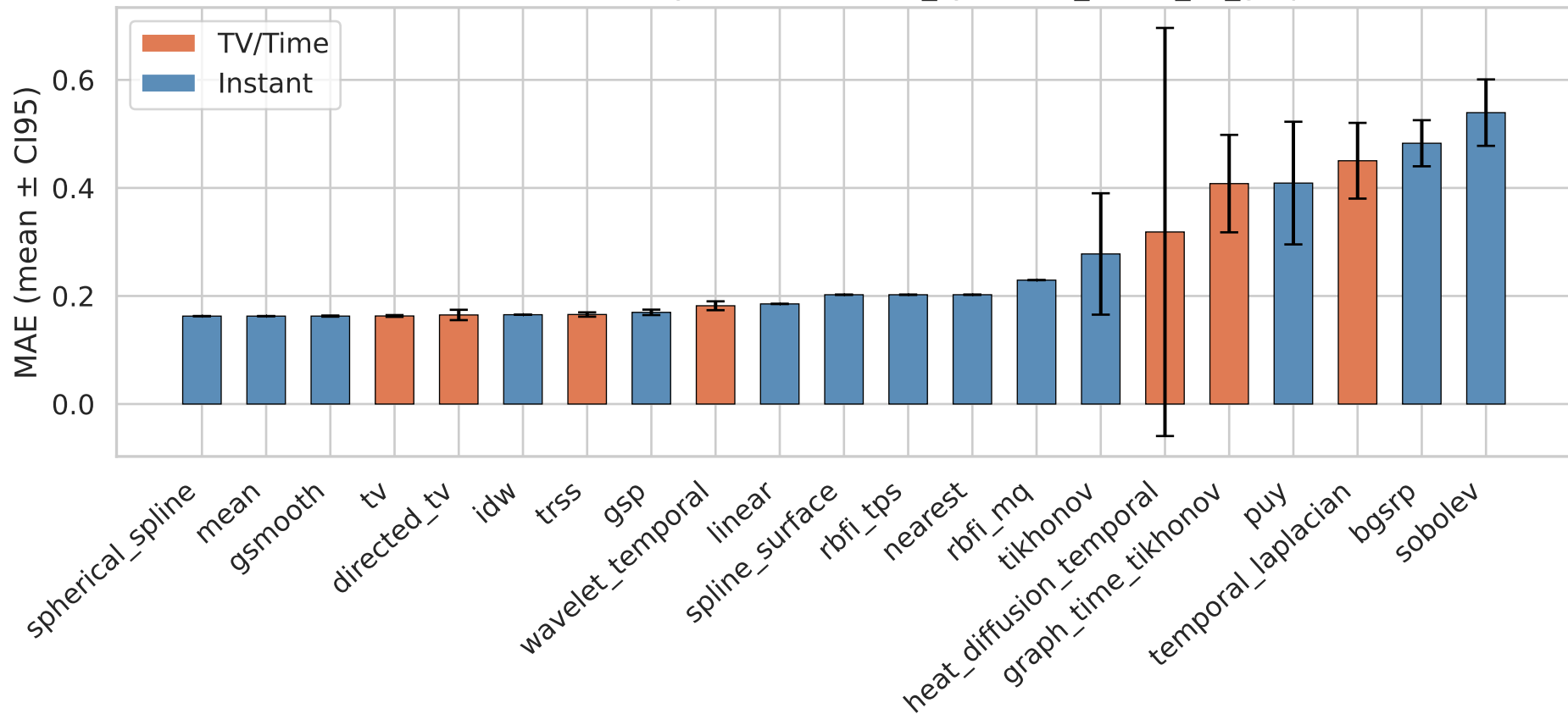
Mean Absolute Error by Method — it17_synthetic_broad_all_graphs
