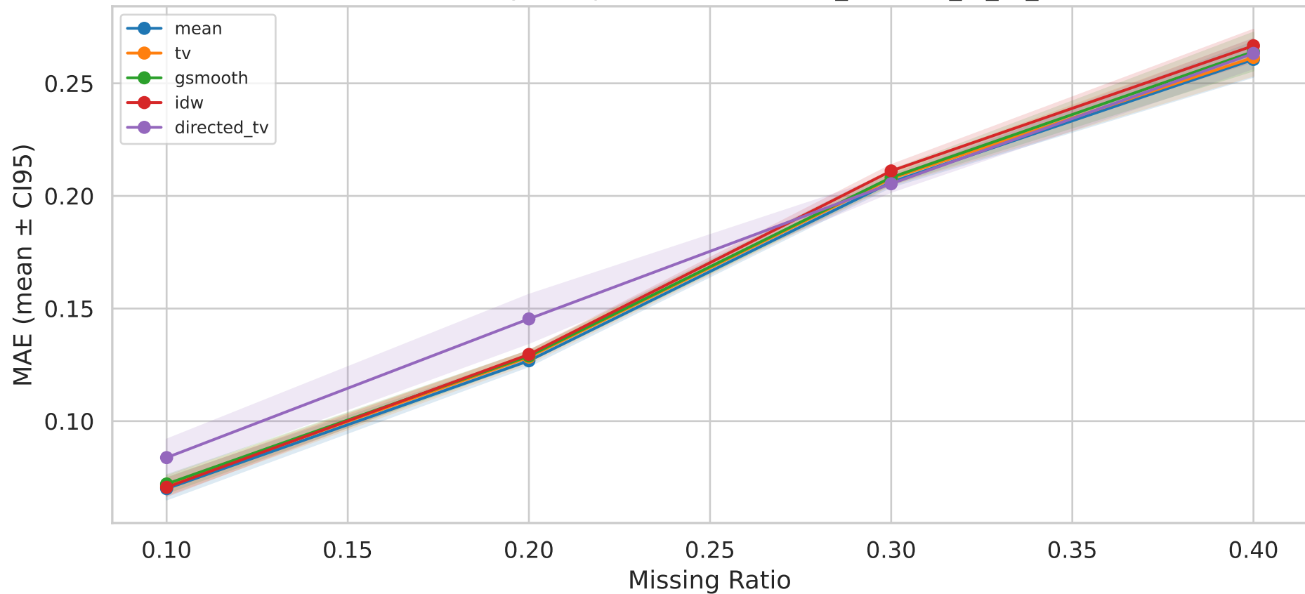
MAE Sensitivity — Top-5 Methods — it18_directed_tv_vs_trss
