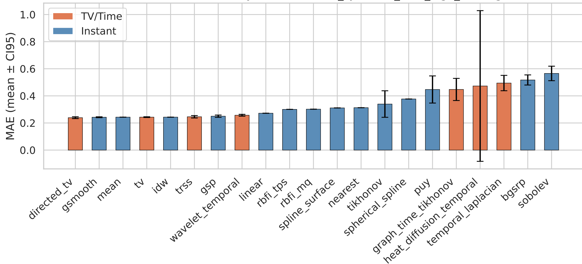
Mean Absolute Error by Method — it19_synthetic_beta_high_missing
