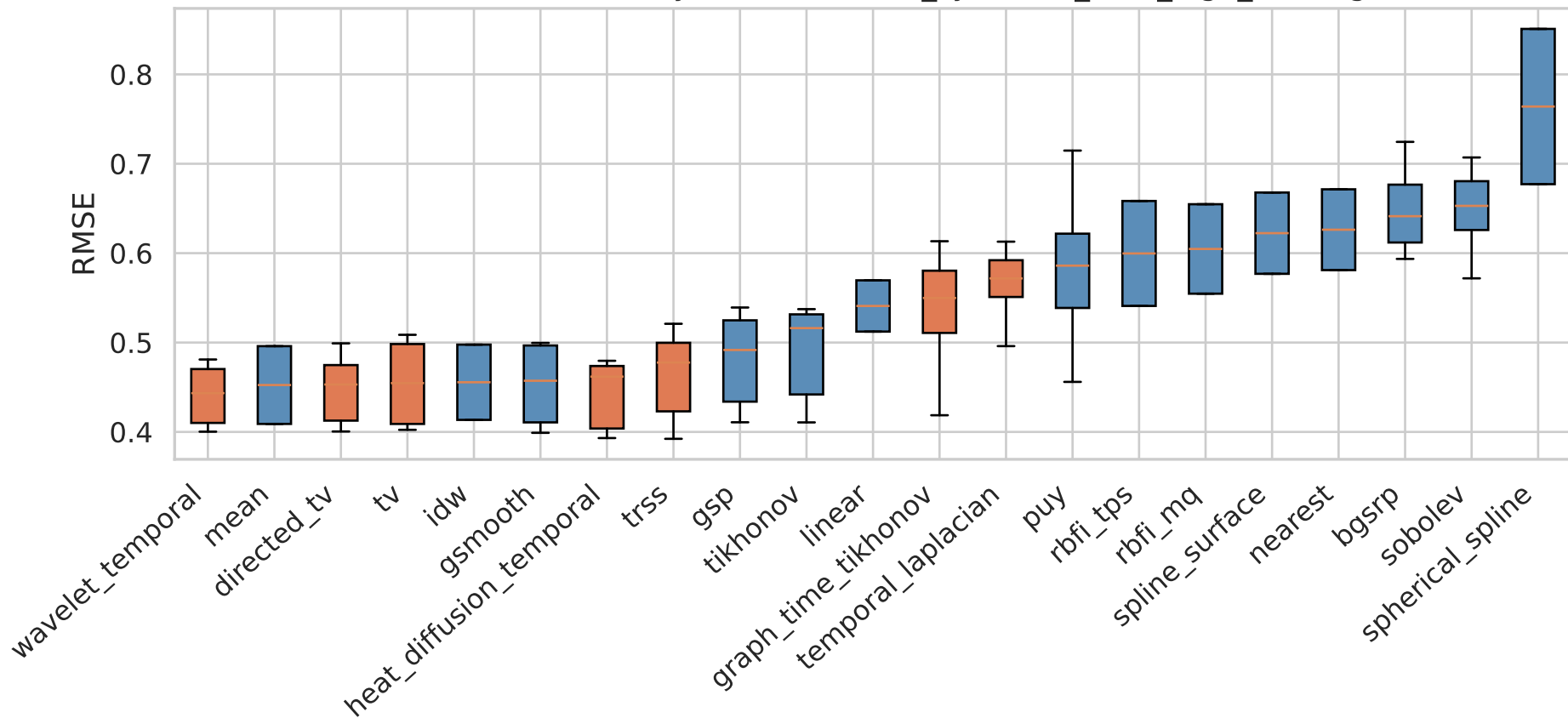
RMSE Distribution by Method — it19_synthetic_beta_high_missing
