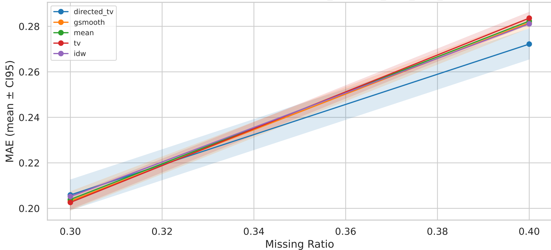
MAE Sensitivity — Top-5 Methods — it19_synthetic_beta_high_missing
