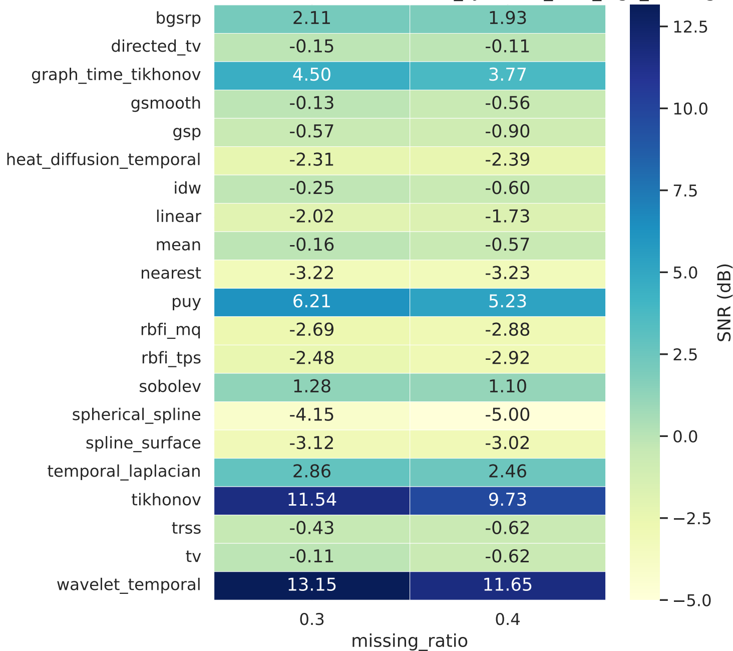
Mean SNR — Method × Scenario — it19_synthetic_beta_high_missing
