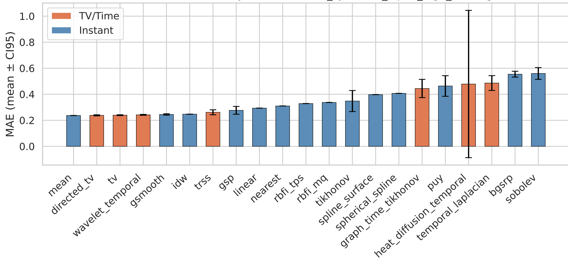
Mean Absolute Error by Method — it20_synthetic_alpha_high_missing
