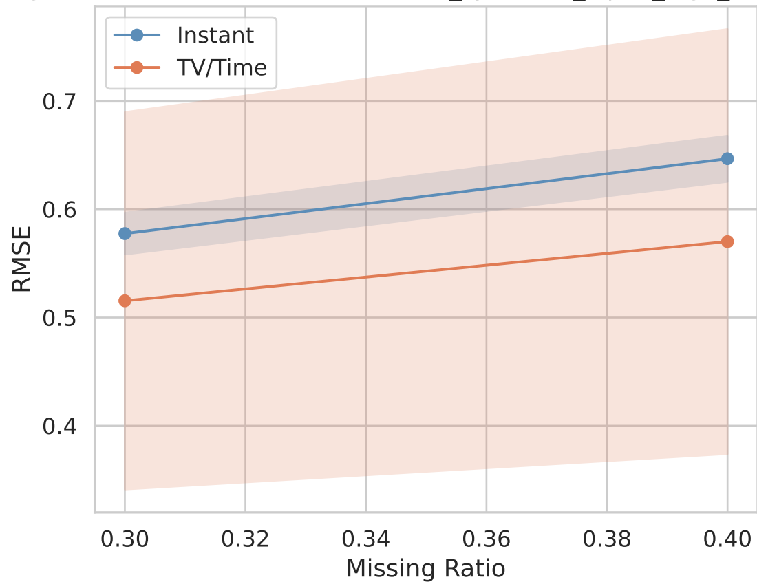
RMSE — TV/Time vs Instant — it20_synthetic_alpha_high_missing
