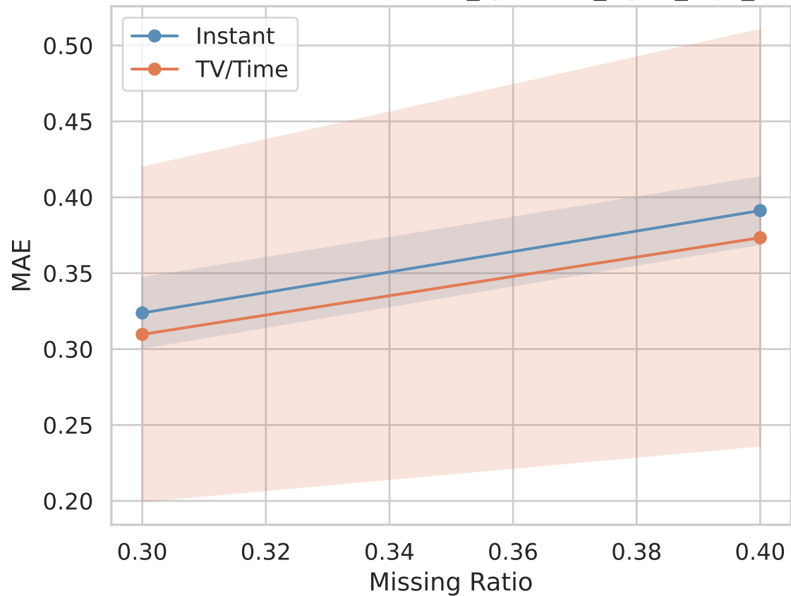
MAE — TV/Time vs Instant — it20_synthetic_alpha_high_missing
