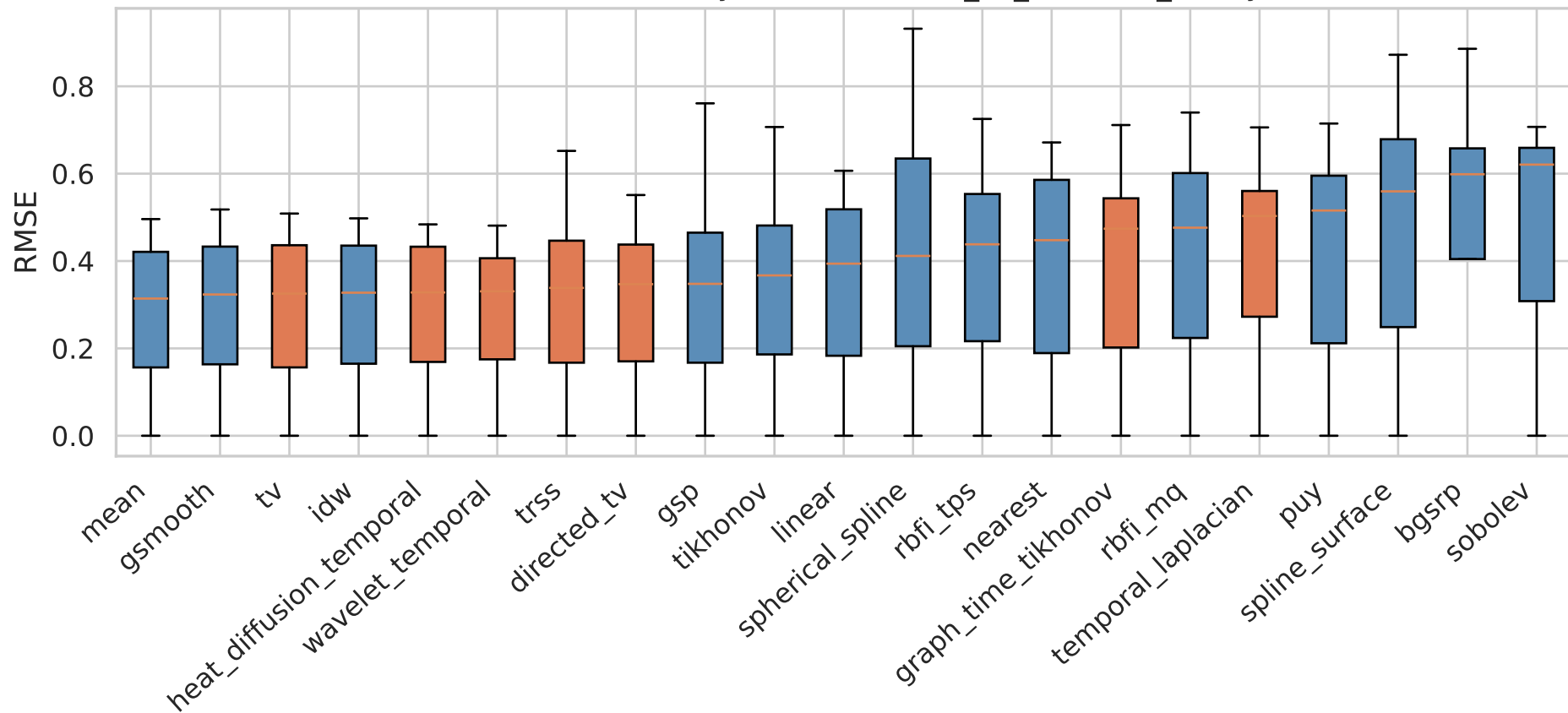
RMSE Distribution by Method — it21_all_datasets_family
