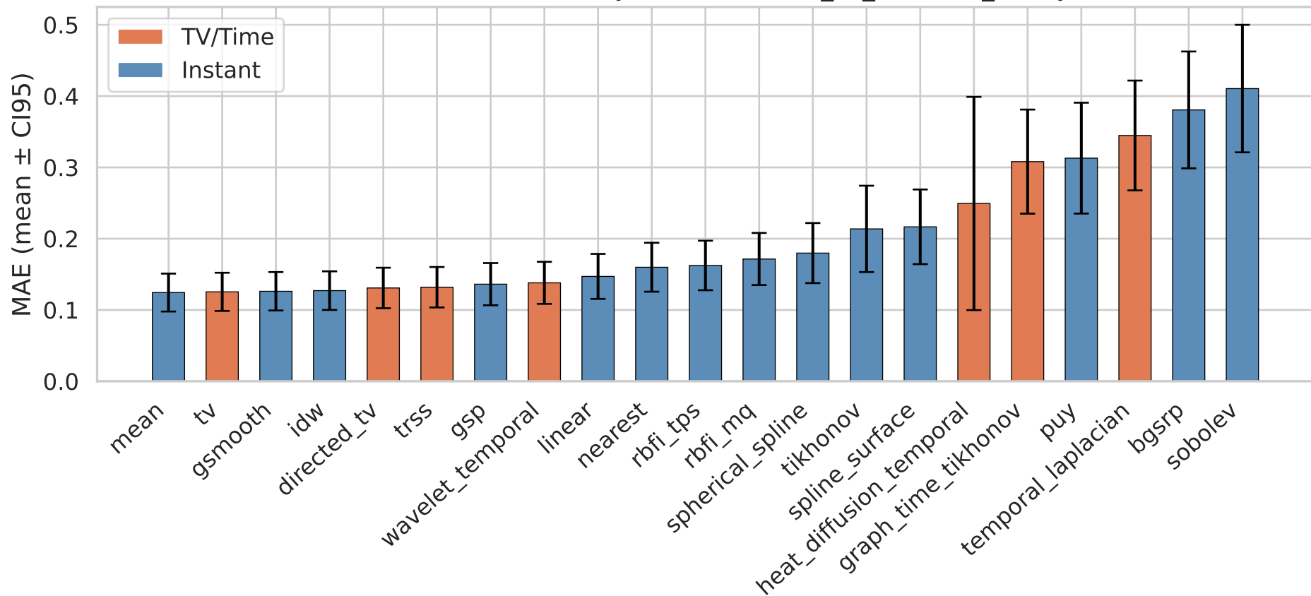
Mean Absolute Error by Method — it21_all_datasets_family
