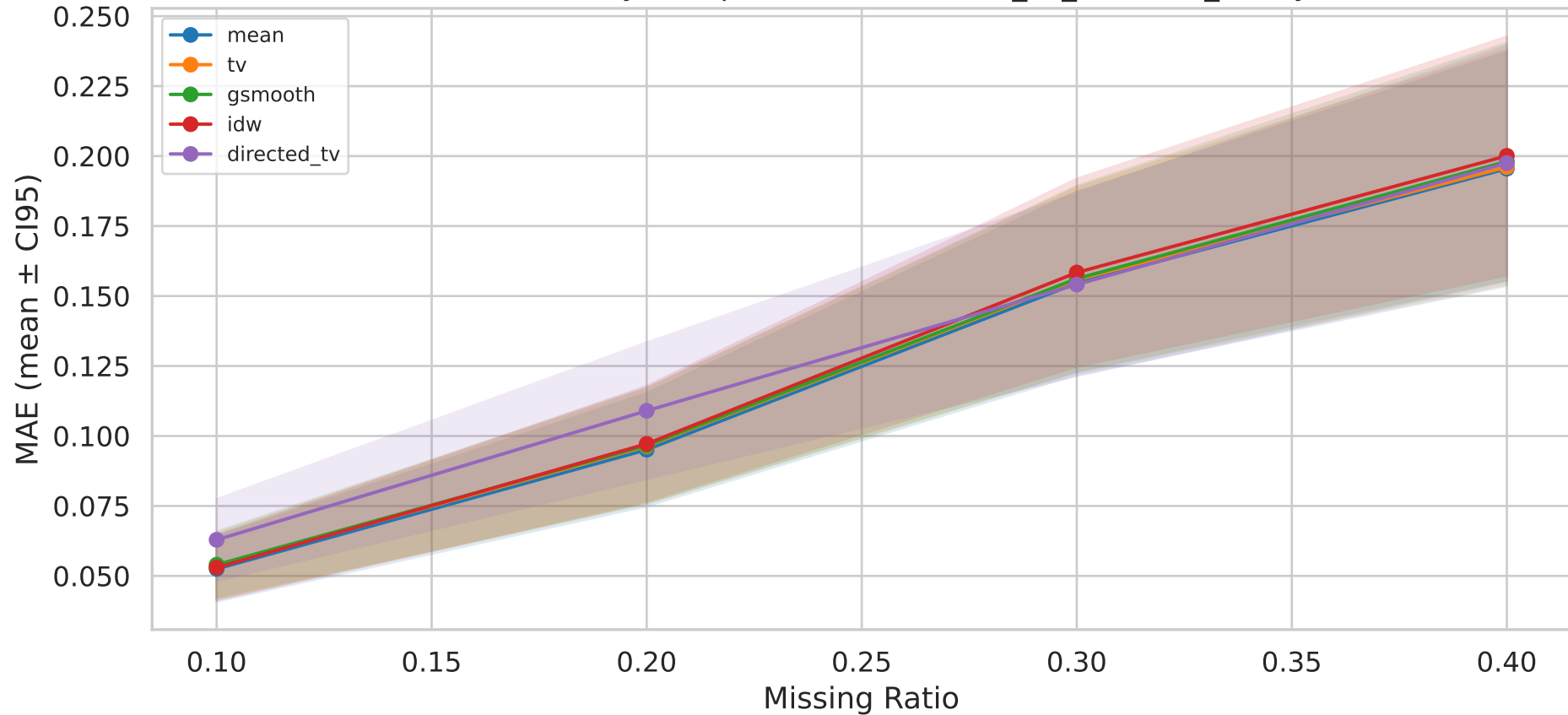
MAE Sensitivity — Top-5 Methods — it21_all_datasets_family
