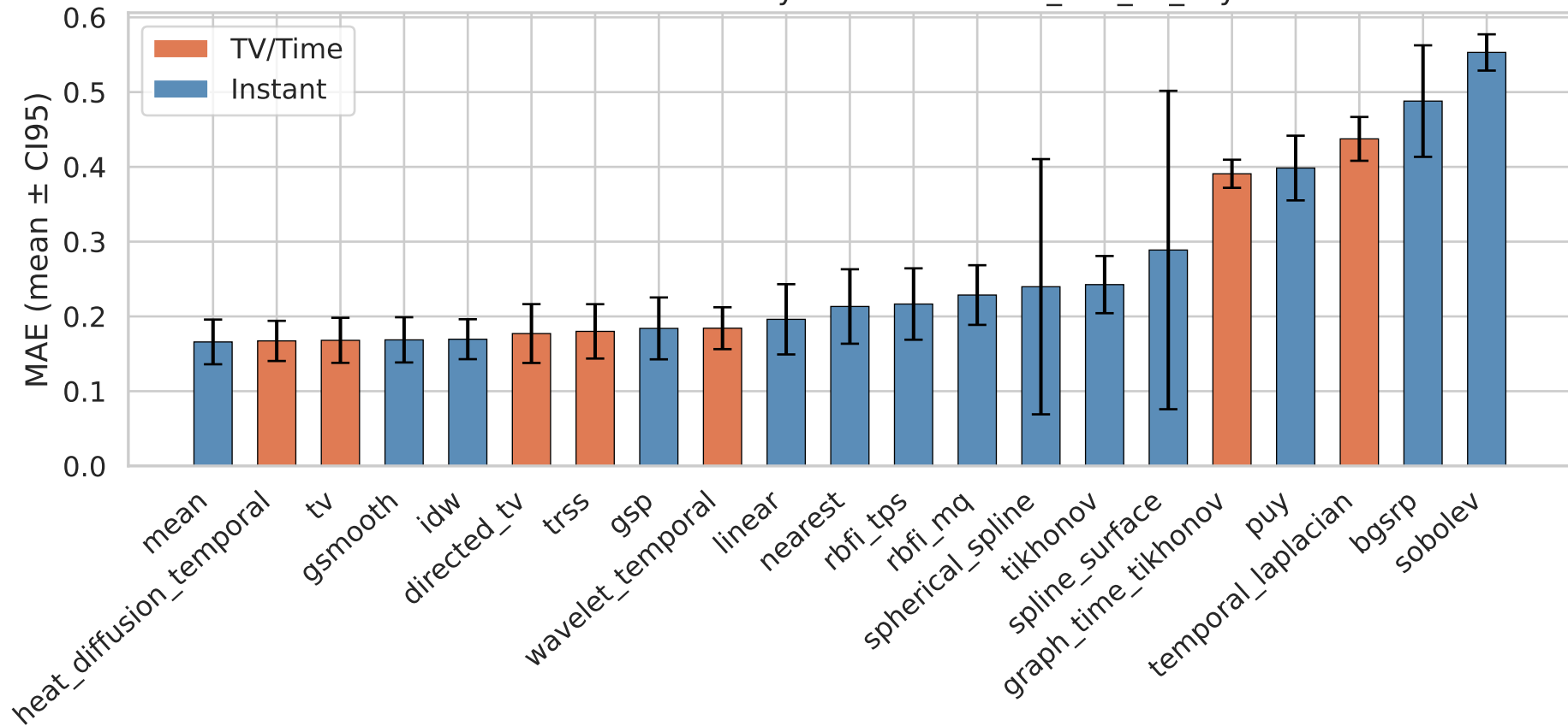
Mean Absolute Error by Method — it22b_knn_k3_3syn
