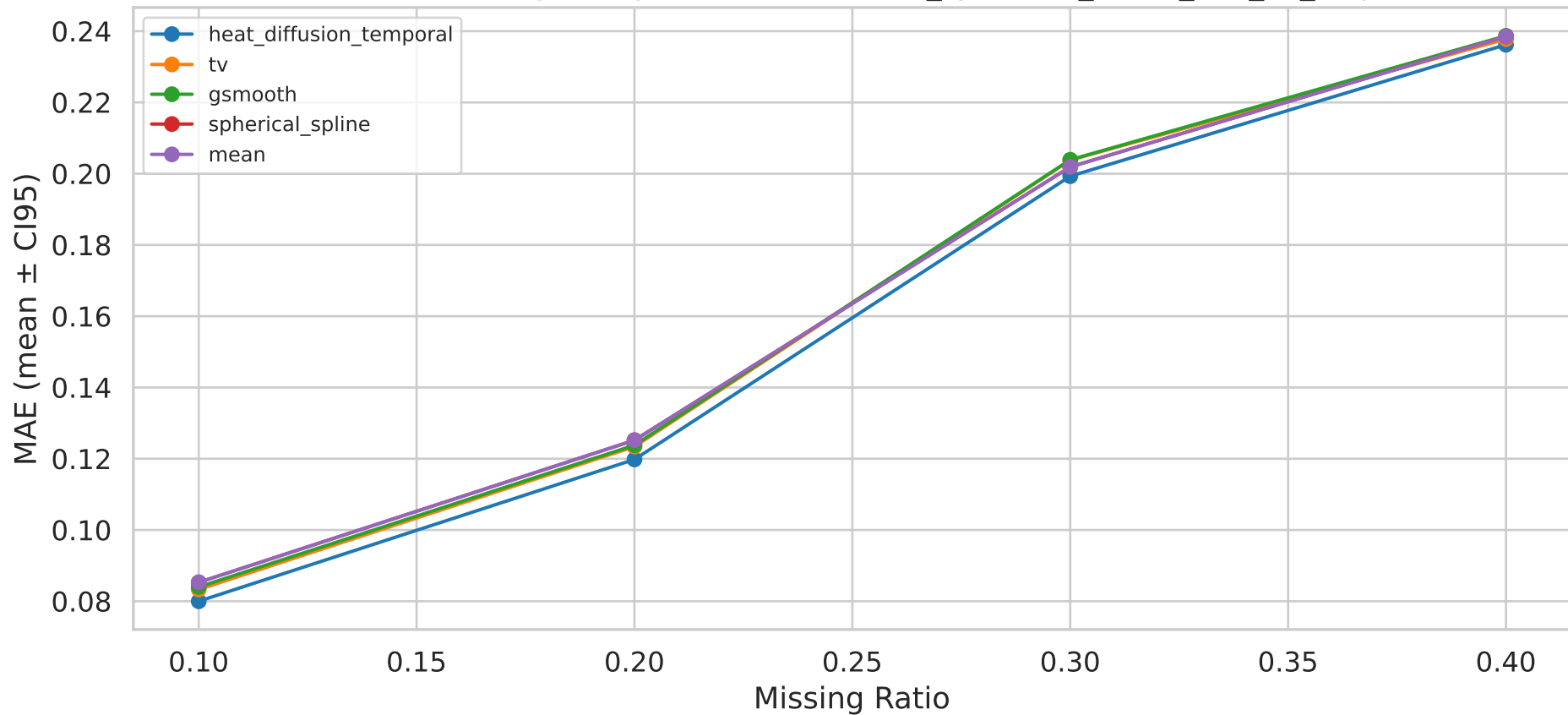
MAE Sensitivity — Top-5 Methods — it22_synthetic_broad_knn_k3_only
