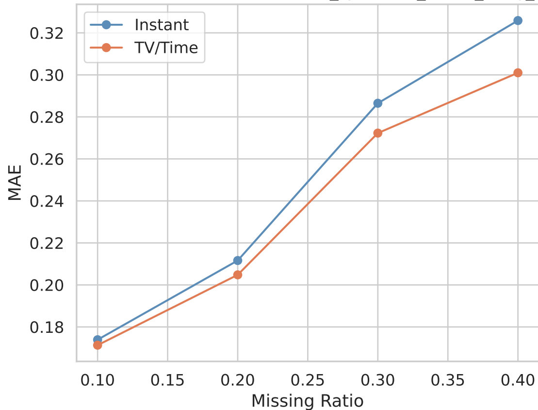
MAE — TV/Time vs Instant — it23_synthetic_broad_knng_only
