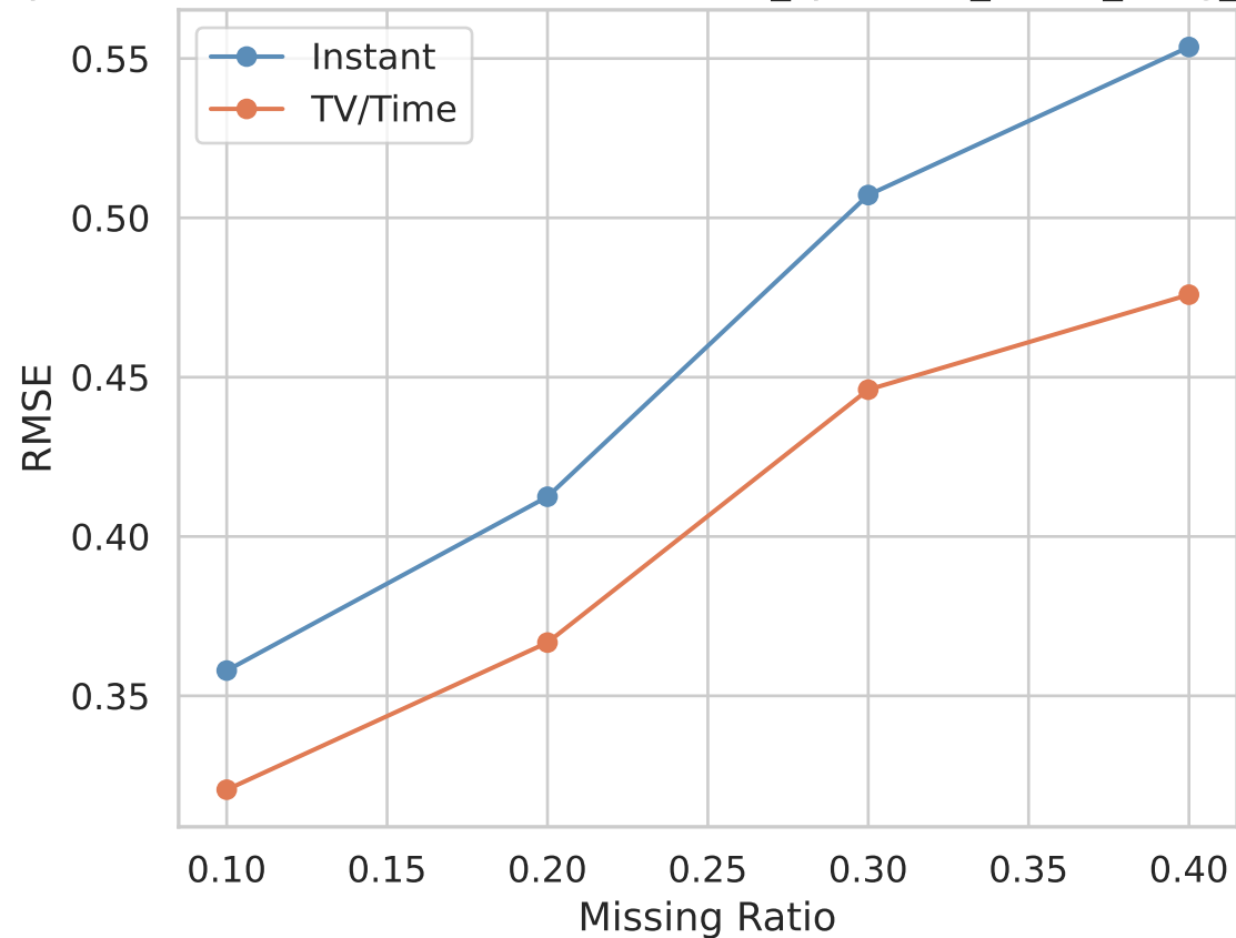
RMSE — TV/Time vs Instant — it23_synthetic_broad_knng_or
