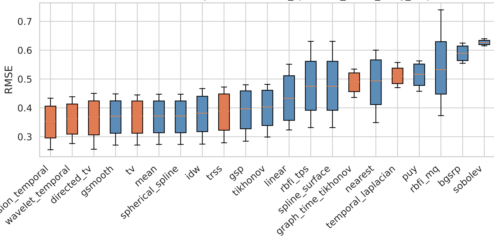
RMSE Distribution by Method — it23_synthetic_broad_knng_only
