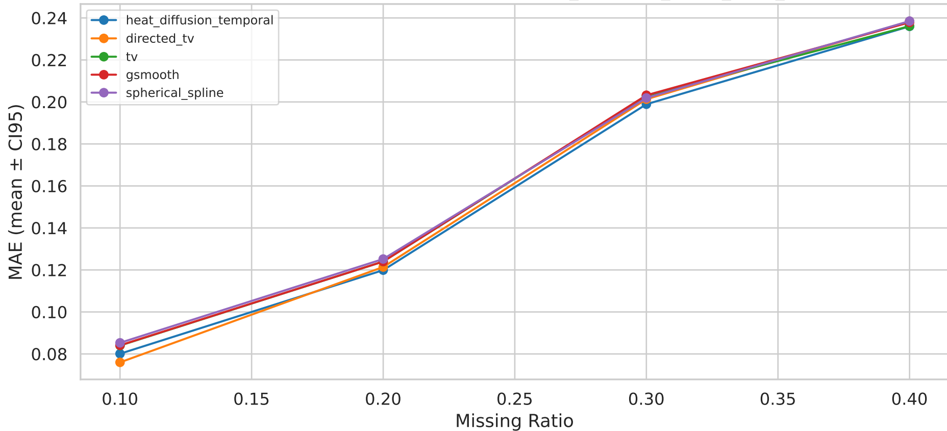
MAE Sensitivity — Top-5 Methods — it23_synthetic_broad_knng_only
