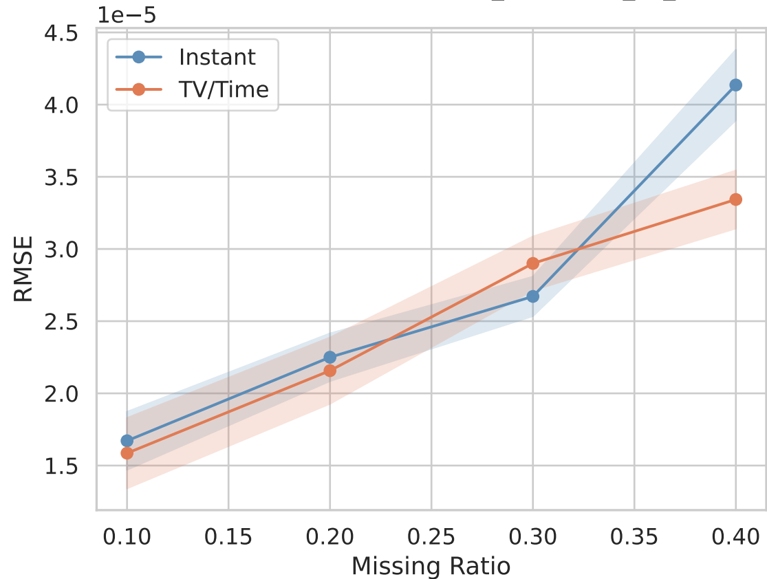
RMSE — TV/Time vs Instant — it24_physionet_all_scenarios
