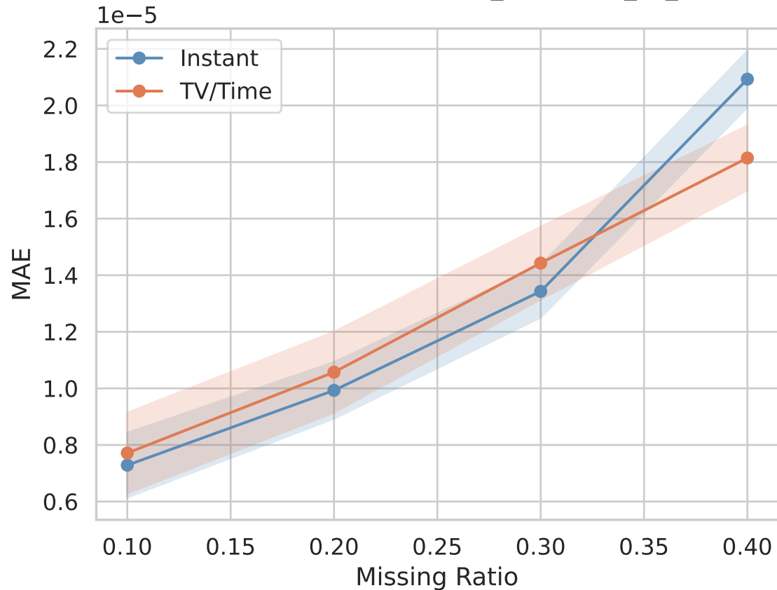
MAE — TV/Time vs Instant — it24_physionet_all_scenarios
