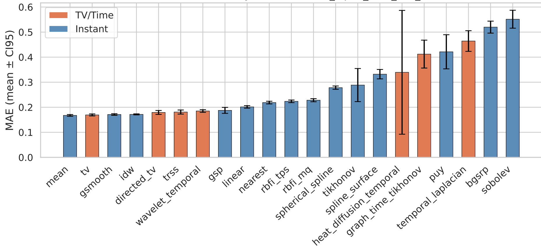
Mean Absolute Error by Method — it25_alpha_beta_two_bands
