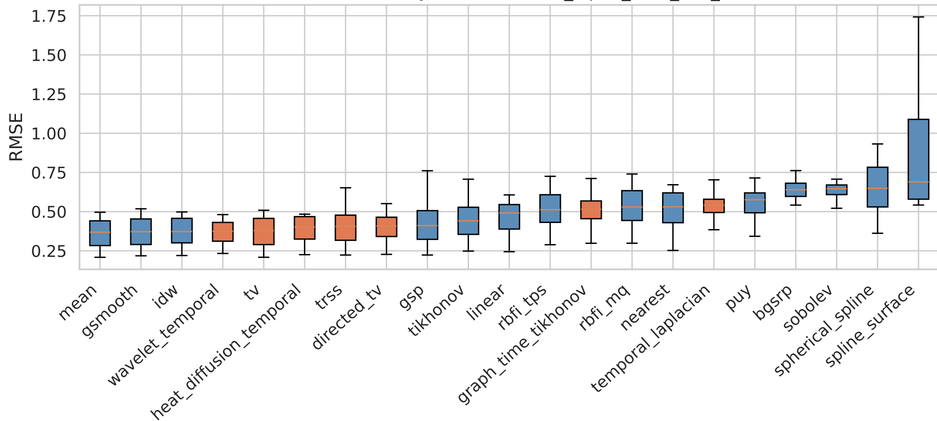
RMSE Distribution by Method — it25_alpha_beta_two_bands
